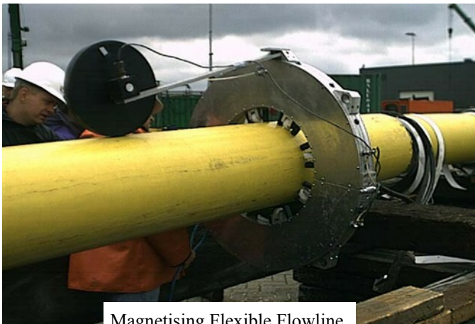
Magnetising Flexible Flowline
